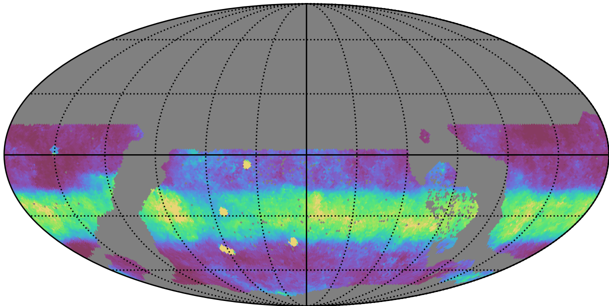
early_u_fpextra3.0_v3.4_10yrs WFD z band: Median normairmass
