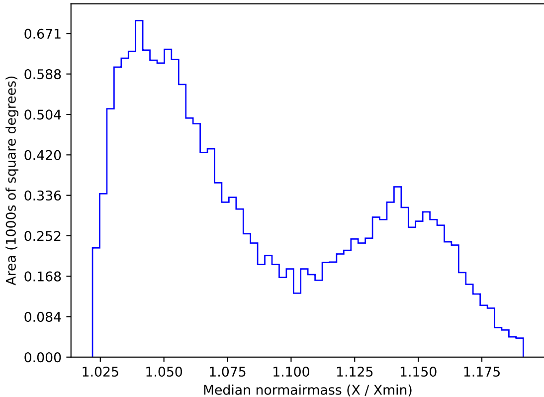
early_u_fpextra3.0_v3.4_10yrs WFD z band: Median normairmass
