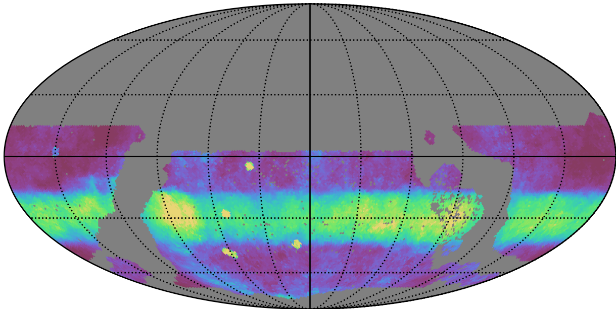
early_u_fpextra3.0_v3.4_10yrs WFD r band: Median normairmass
