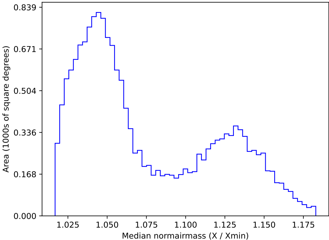
early_u_fpextra3.0_v3.4_10yrs WFD r band: Median normairmass
