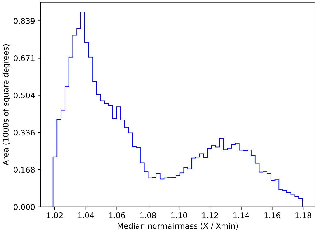
early_u_fpextra3.0_v3.4_10yrs WFD i band: Median normairmass
