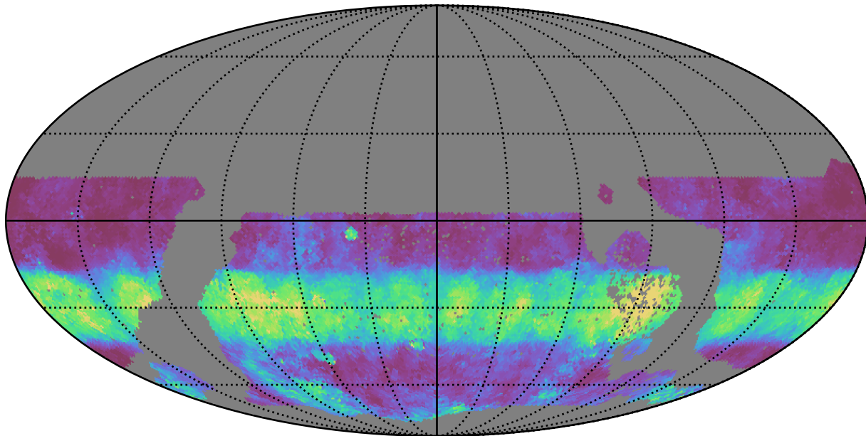
early_u_fpextra3.0_v3.4_10yrs WFD g band: Median normairmass
