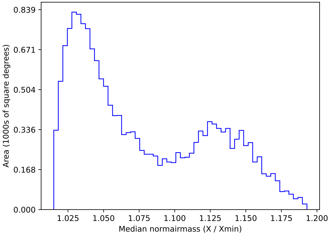
early_u_fpextra3.0_v3.4_10yrs WFD g band: Median normairmass
