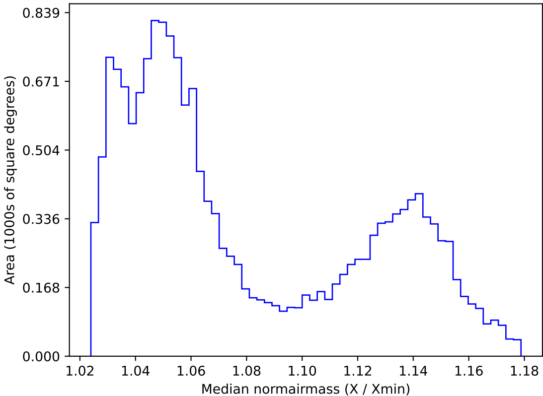
early_u_fpextra3.0_v3.4_10yrs WFD all bands: Median normairmass
