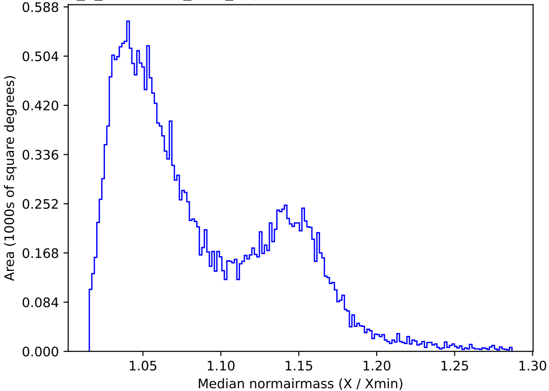
early_u_fpextra3.0_v3.4_10yrs All sky z band: Median normairmass
