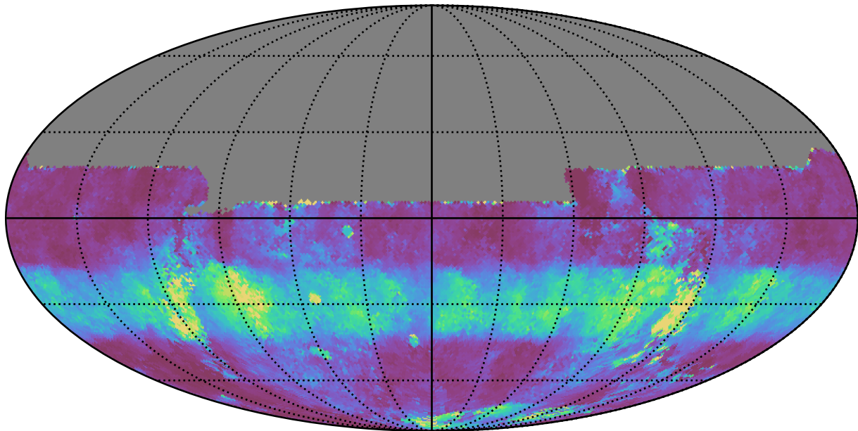
early_u_fpextra3.0_v3.4_10yrs All sky u band: Median normairmass
