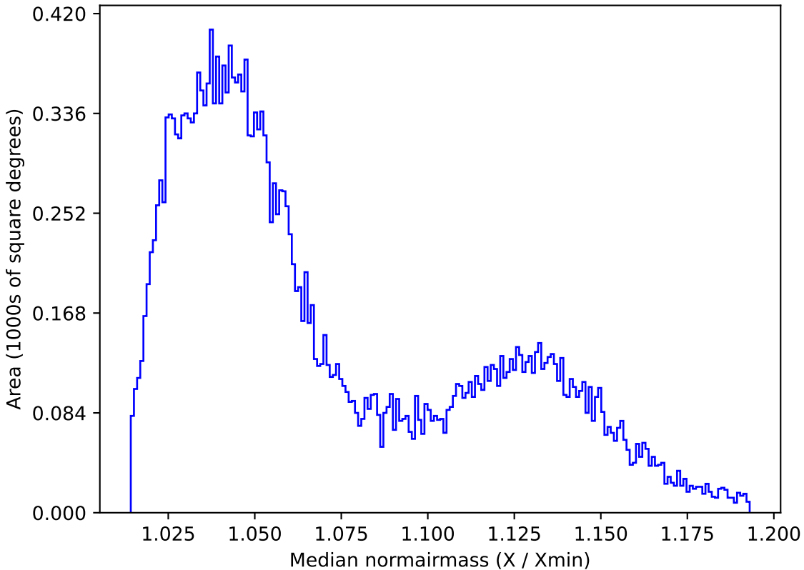
early_u_fpextra3.0_v3.4_10yrs All sky r band: Median normairmass
