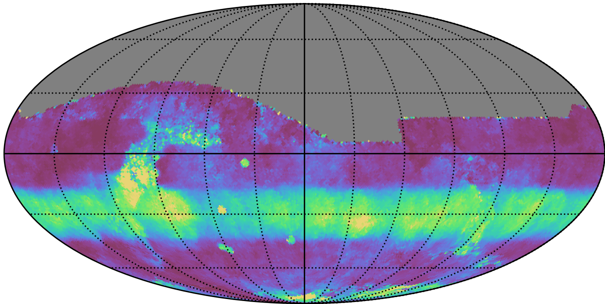
early_u_fpextra3.0_v3.4_10yrs All sky i band: Median normairmass
