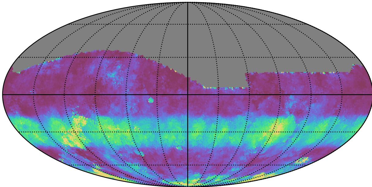
early_u_fpextra3.0_v3.4_10yrs All sky g band: Median normairmass
