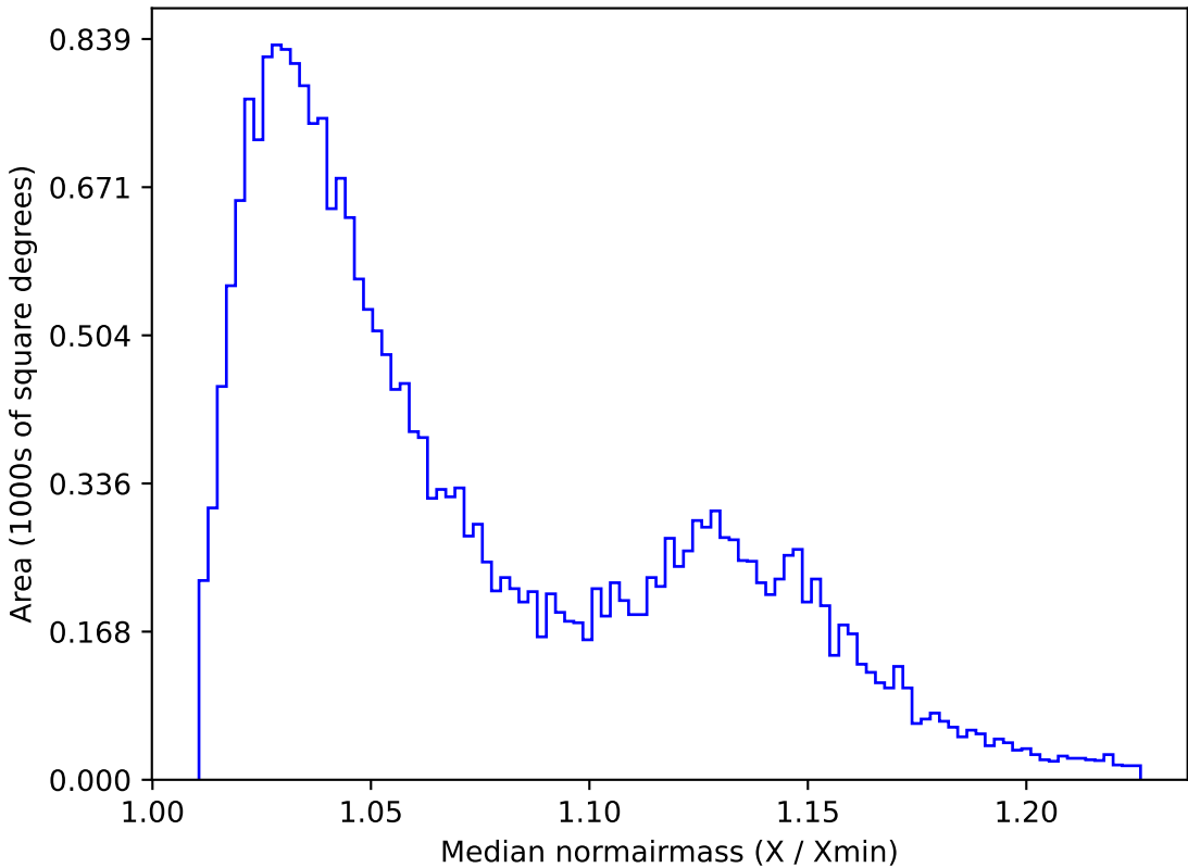
early_u_fpextra3.0_v3.4_10yrs All sky g band: Median normairmass
