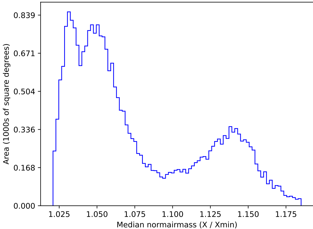
early_u_fpextra3.0_v3.4_10yrs All sky all bands: Median normairmass
