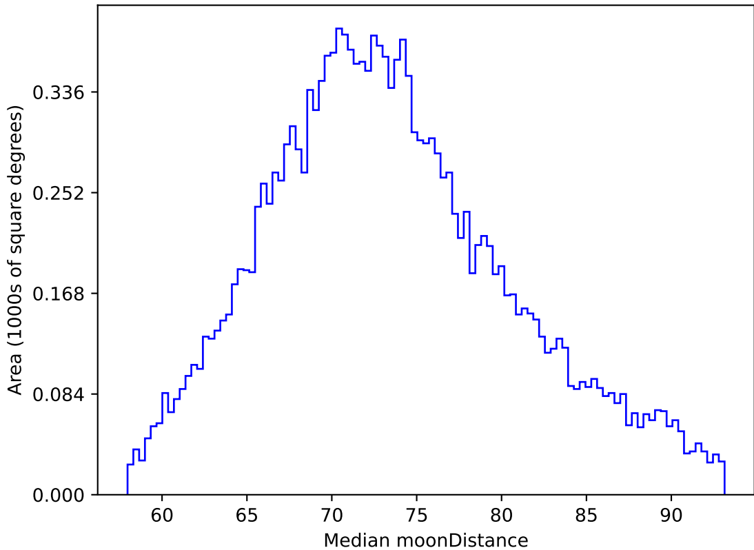
early_u_fpextra3.0_v3.4_10yrs WFD z band: Median moonDistance
