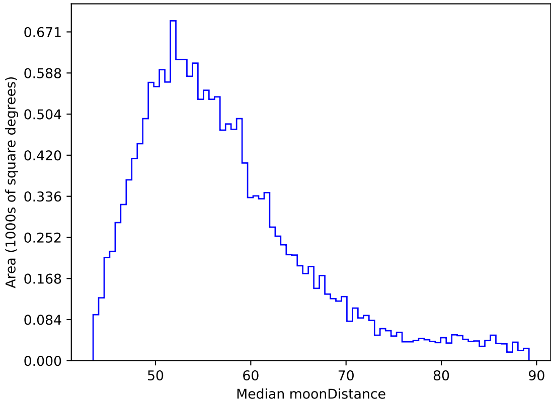
early_u_fpextra3.0_v3.4_10yrs WFD y band: Median moonDistance
