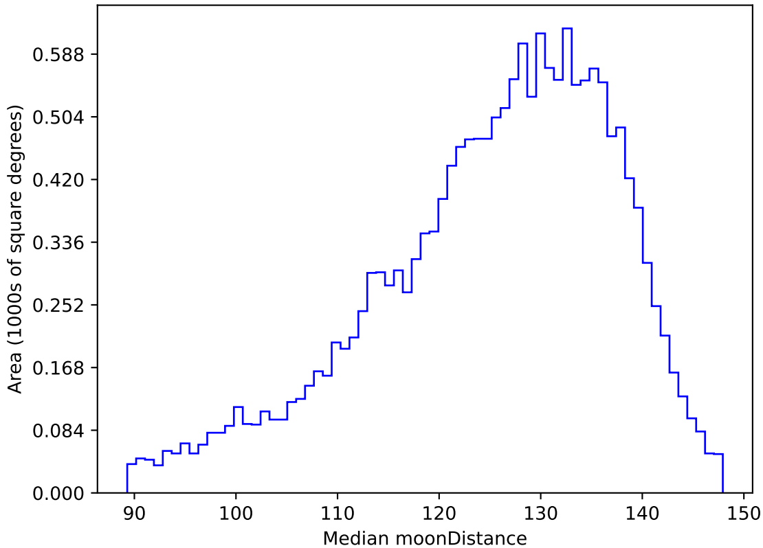
early_u_fpextra3.0_v3.4_10yrs WFD u band: Median moonDistance
