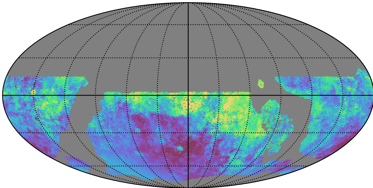
early_u_fpextra3.0_v3.4_10yrs WFD i band: Median moonDistance
