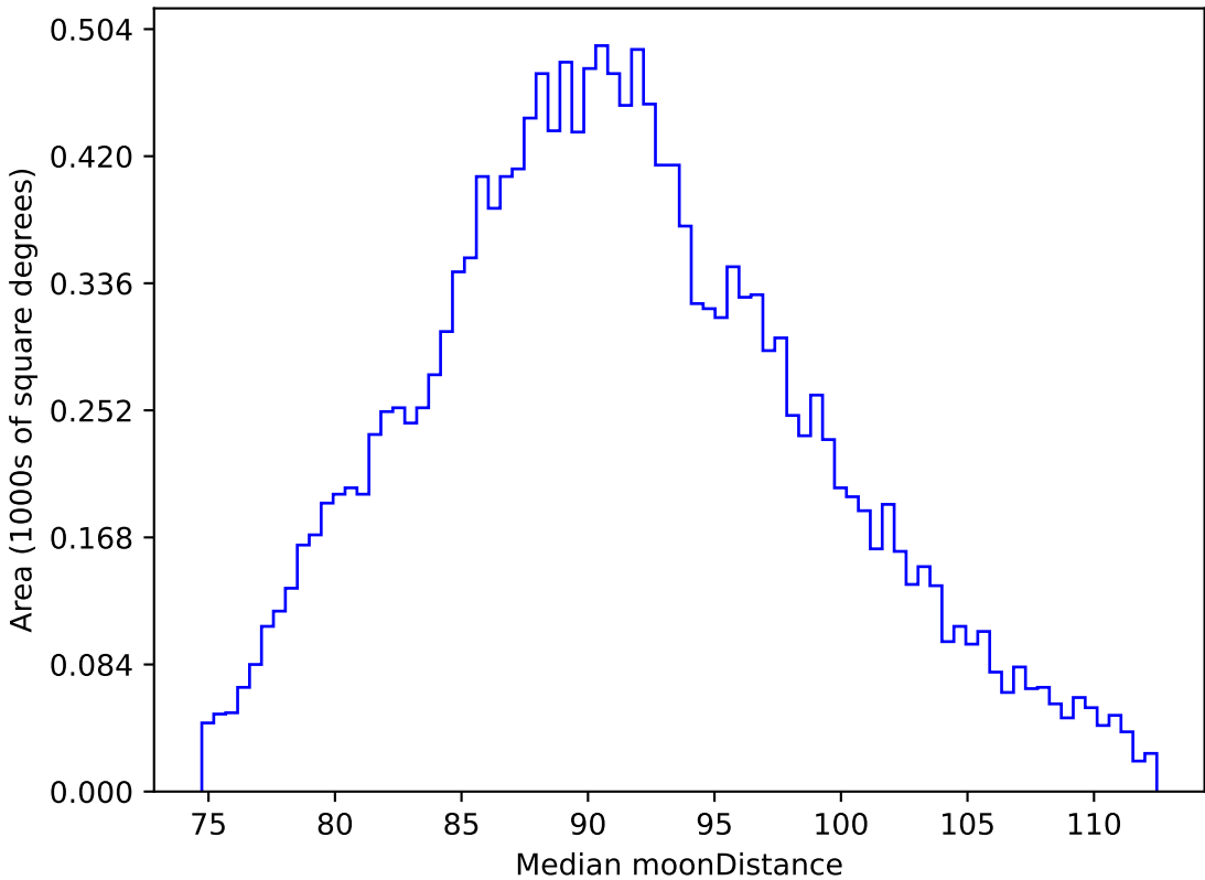
early_u_fpextra3.0_v3.4_10yrs WFD i band: Median moonDistance
