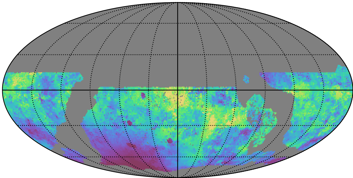
early_u_fpextra3.0_v3.4_10yrs WFD g band: Median moonDistance
