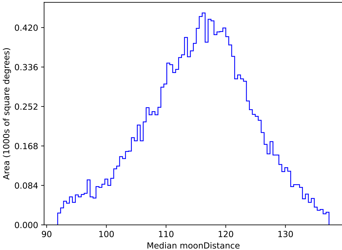
early_u_fpextra3.0_v3.4_10yrs WFD g band: Median moonDistance
