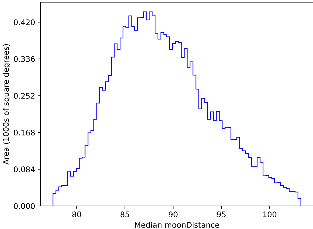
early_u_fpextra3.0_v3.4_10yrs WFD all bands: Median moonDistance
