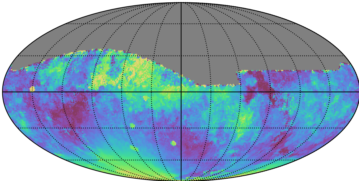
early_u_fpextra3.0_v3.4_10yrs All sky z band: Median moonDistance
