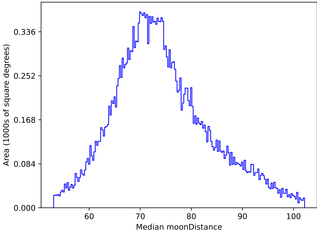
early_u_fpextra3.0_v3.4_10yrs All sky z band: Median moonDistance
