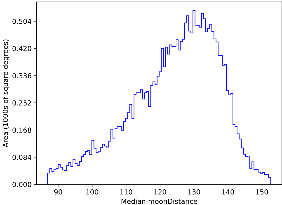
early_u_fpextra3.0_v3.4_10yrs All sky u band: Median moonDistance
