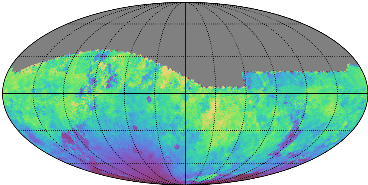
early_u_fpextra3.0_v3.4_10yrs All sky r band: Median moonDistance
