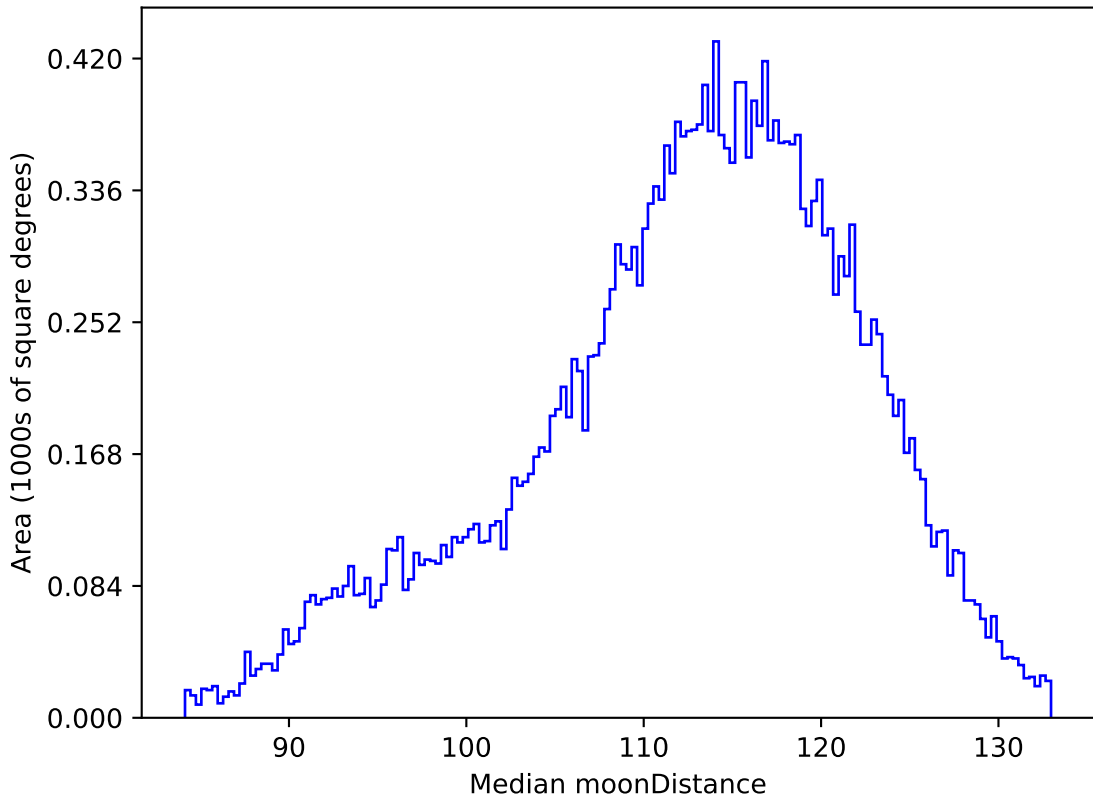
early_u_fpextra3.0_v3.4_10yrs All sky r band: Median moonDistance
