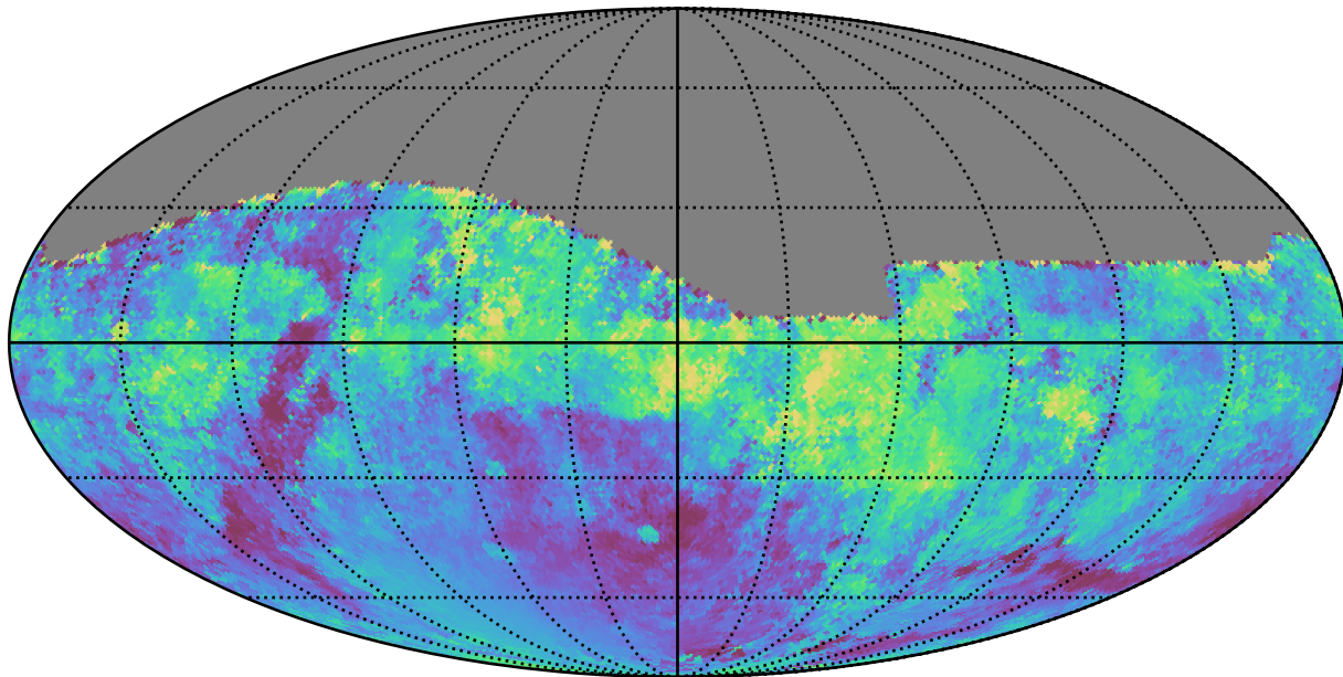
early_u_fpextra3.0_v3.4_10yrs All sky i band: Median moonDistance
