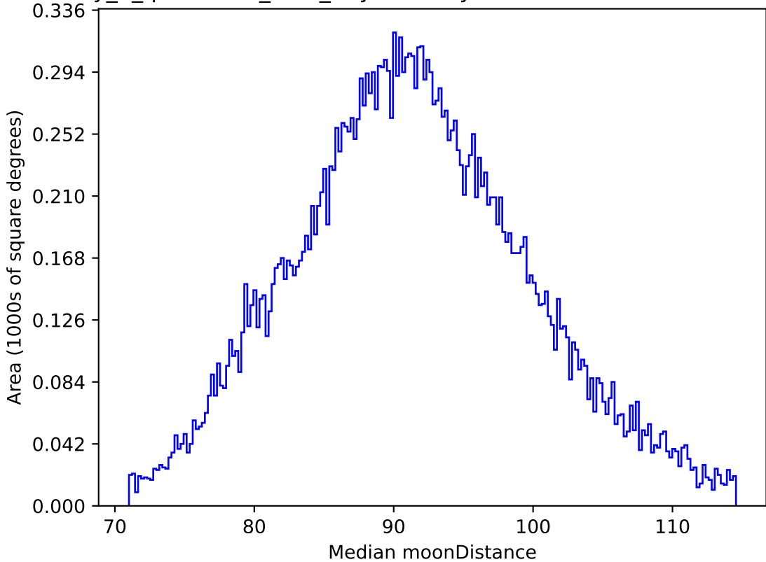
early_u_fpextra3.0_v3.4_10yrs All sky i band: Median moonDistance
