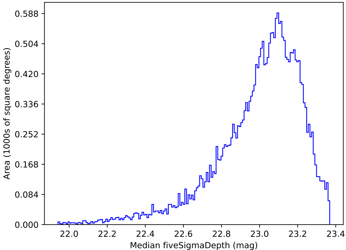
early_u_fpextra3.0_v3.4_10yrs Yr 1 z band: Median fiveSigmaDepth
