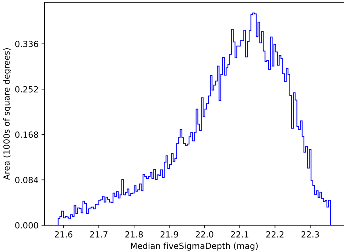
early_u_fpextra3.0_v3.4_10yrs Yr 1 y band: Median fiveSigmaDepth
