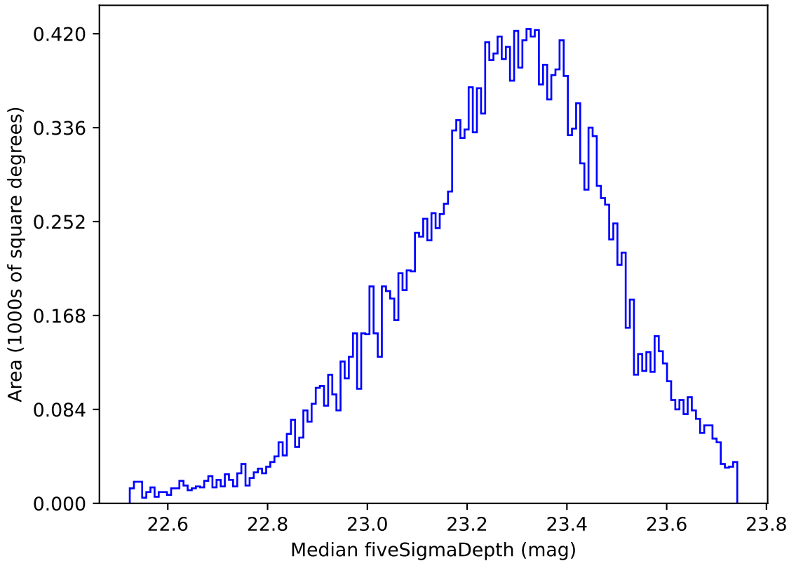
early_u_fpextra3.0_v3.4_10yrs Yr 1 u band: Median fiveSigmaDepth
