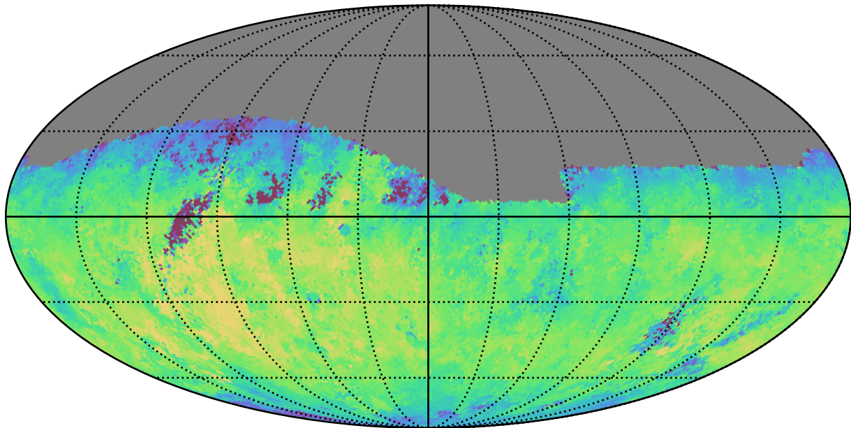
early_u_fpextra3.0_v3.4_10yrs Yr 1 r band: Median fiveSigmaDepth
