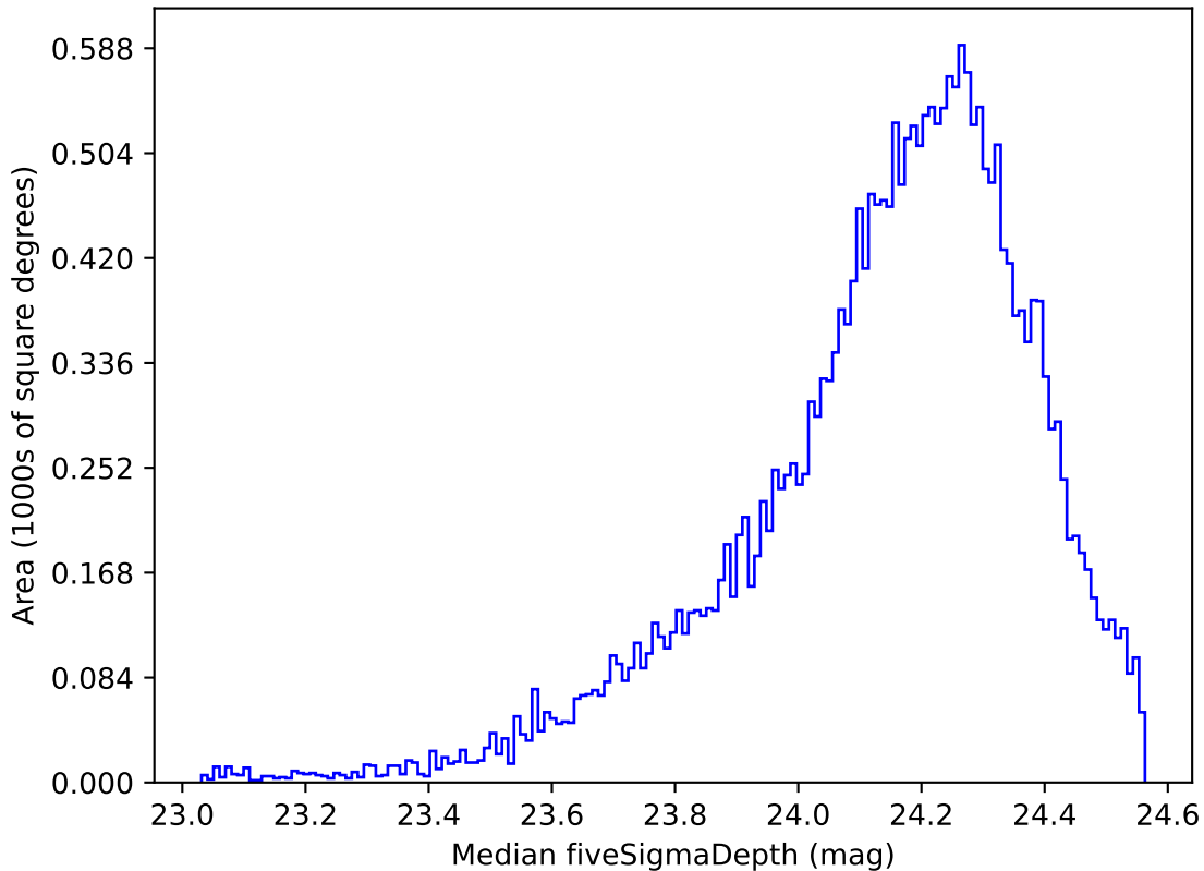
early_u_fpextra3.0_v3.4_10yrs Yr 1 r band: Median fiveSigmaDepth
