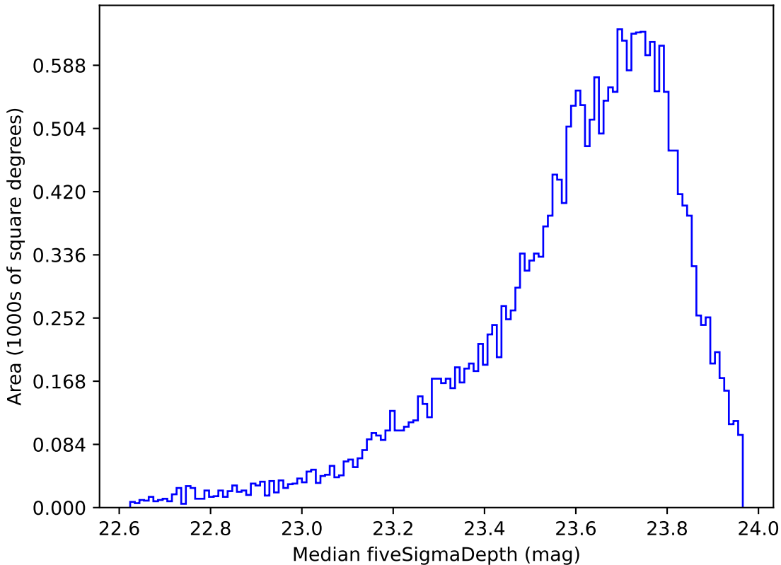
early_u_fpextra3.0_v3.4_10yrs Yr 1 i band: Median fiveSigmaDepth
