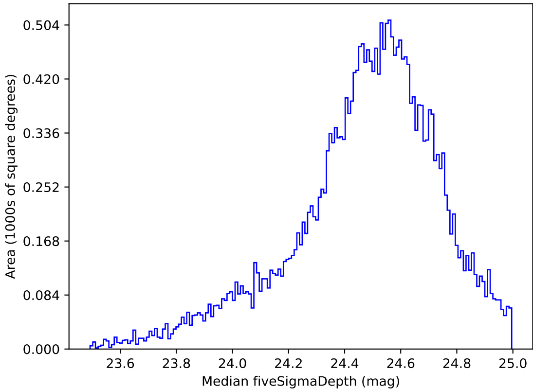
early_u_fpextra3.0_v3.4_10yrs Yr 1 g band: Median fiveSigmaDepth
