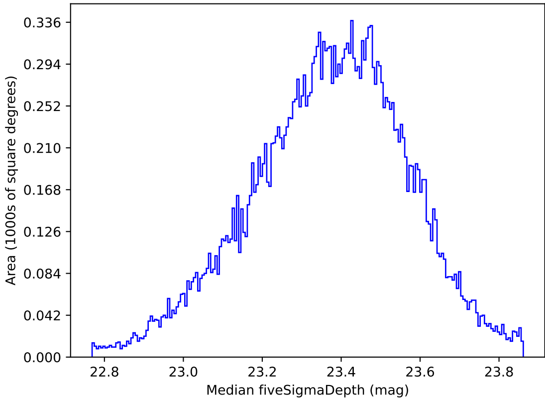
early_u_fpextra3.0_v3.4_10yrs Yr 1 all bands: Median fiveSigmaDepth
