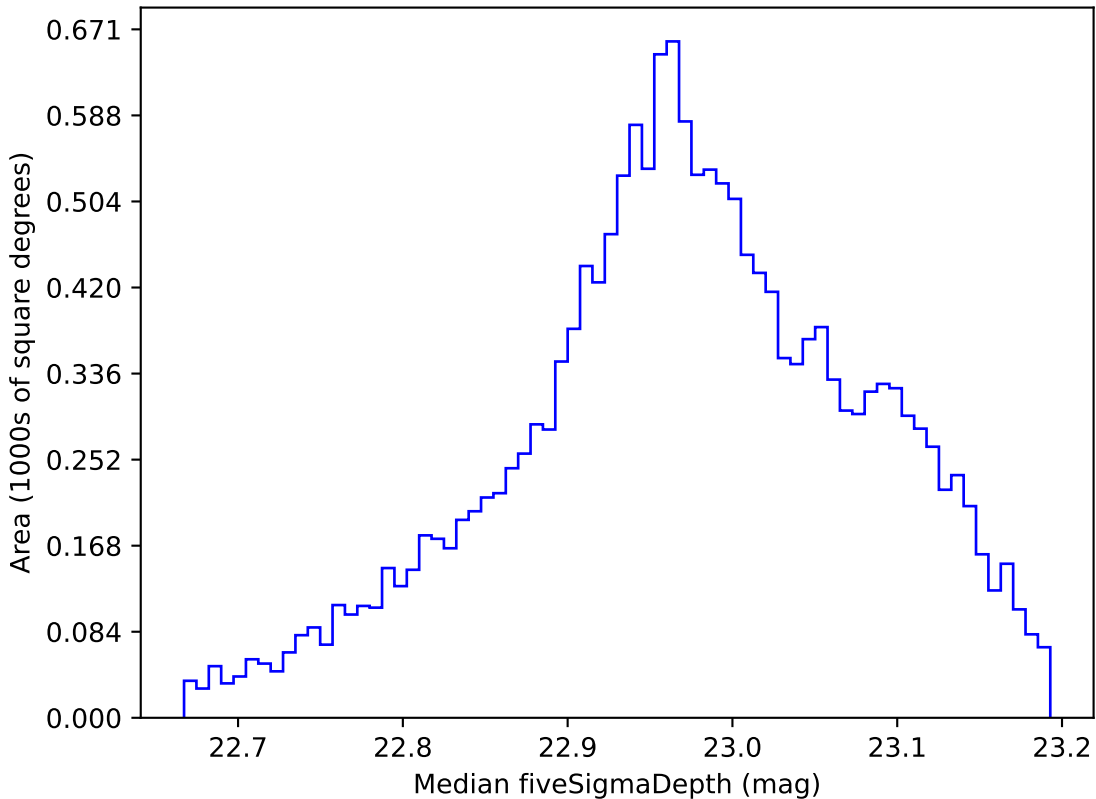
early_u_fpextra3.0_v3.4_10yrs WFD z band: Median fiveSigmaDepth
