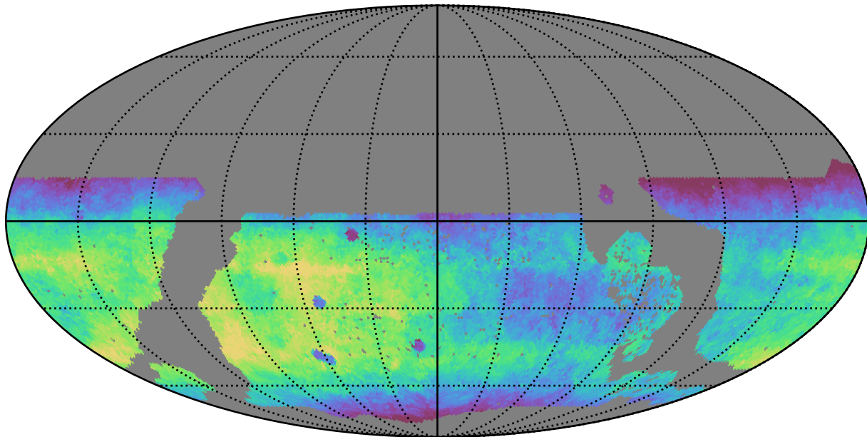
early_u_fpextra3.0_v3.4_10yrs WFD r band: Median fiveSigmaDepth
