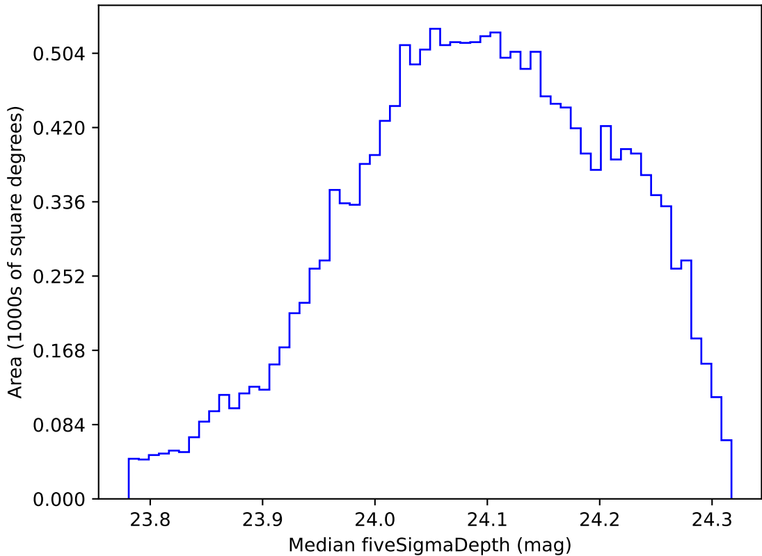
early_u_fpextra3.0_v3.4_10yrs WFD r band: Median fiveSigmaDepth
