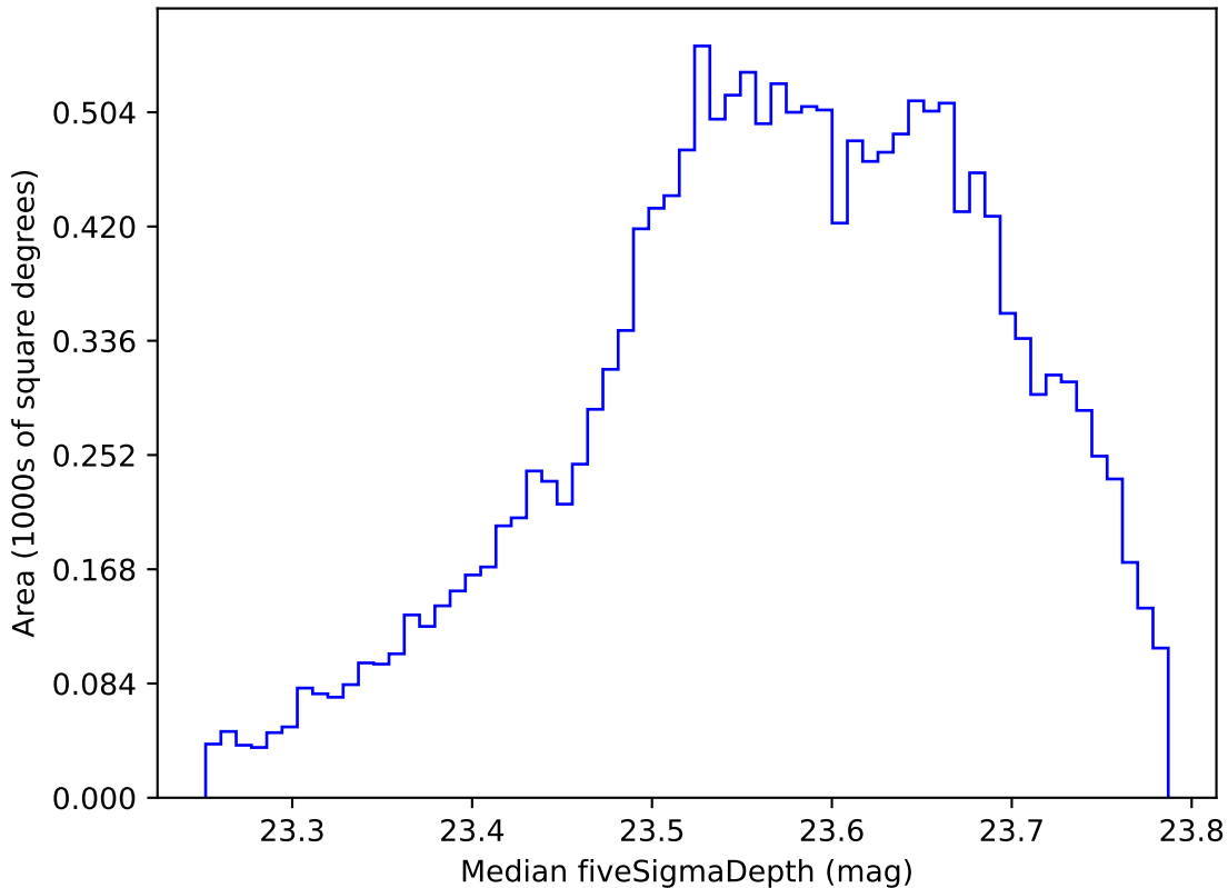
early_u_fpextra3.0_v3.4_10yrs WFD i band: Median fiveSigmaDepth
