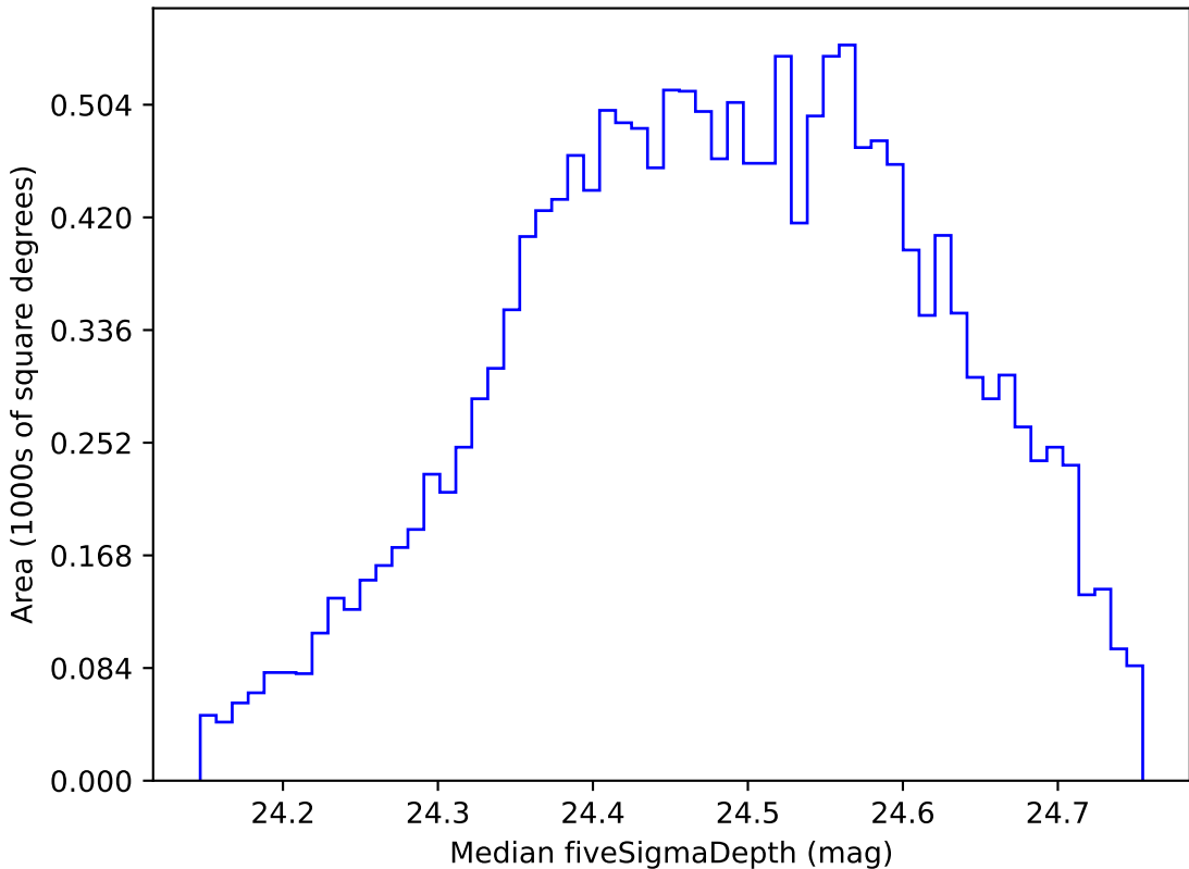
early_u_fpextra3.0_v3.4_10yrs WFD g band: Median fiveSigmaDepth
