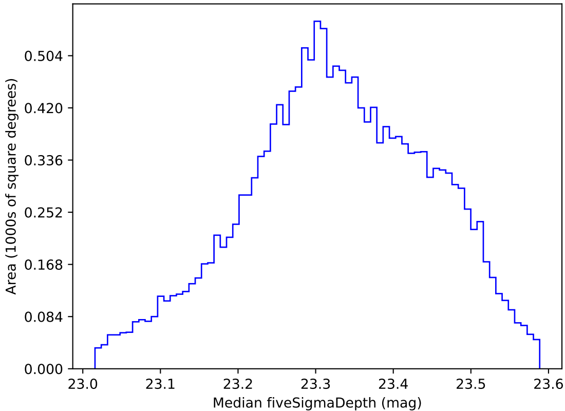
early_u_fpextra3.0_v3.4_10yrs WFD all bands: Median fiveSigmaDepth
