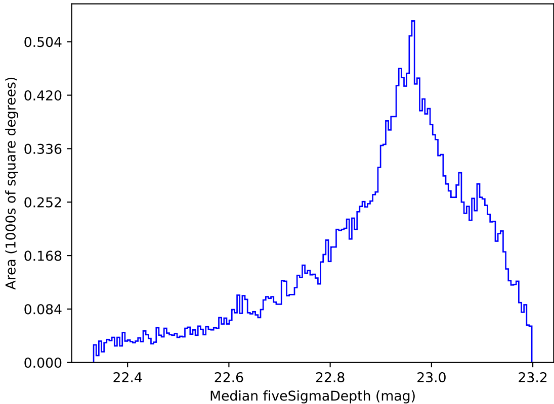
early_u_fpextra3.0_v3.4_10yrs All sky z band: Median fiveSigmaDepth
