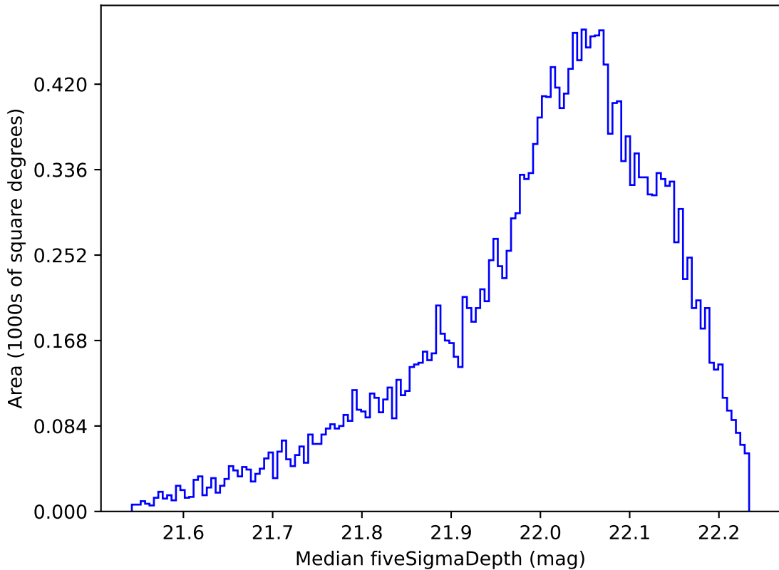
early_u_fpextra3.0_v3.4_10yrs All sky y band: Median fiveSigmaDepth
