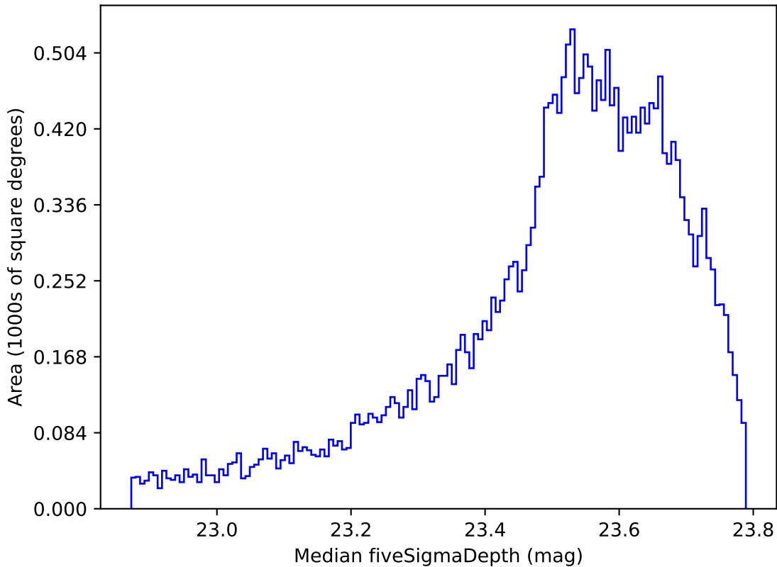
early_u_fpextra3.0_v3.4_10yrs All sky i band: Median fiveSigmaDepth
