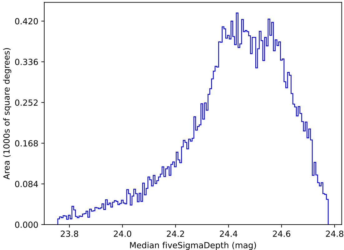
early_u_fpextra3.0_v3.4_10yrs All sky g band: Median fiveSigmaDepth
