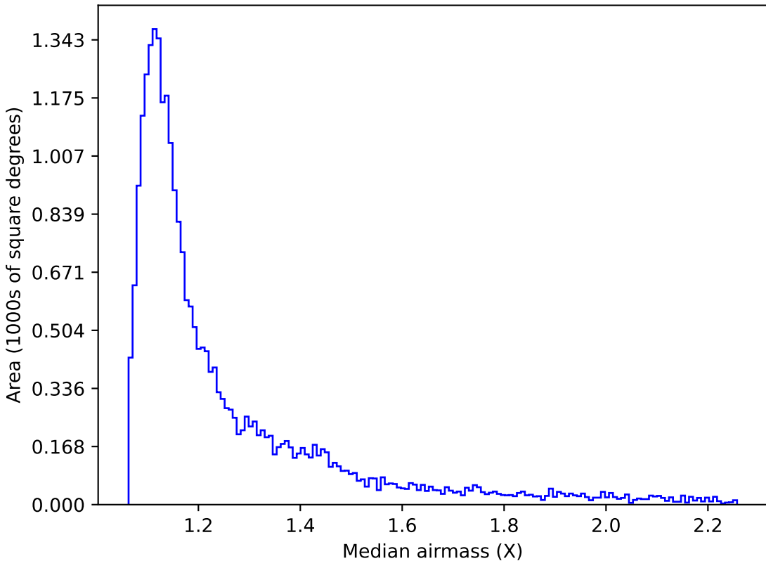
early_u_fpextra3.0_v3.4_10yrs Yr 1 z band: Median airmass
