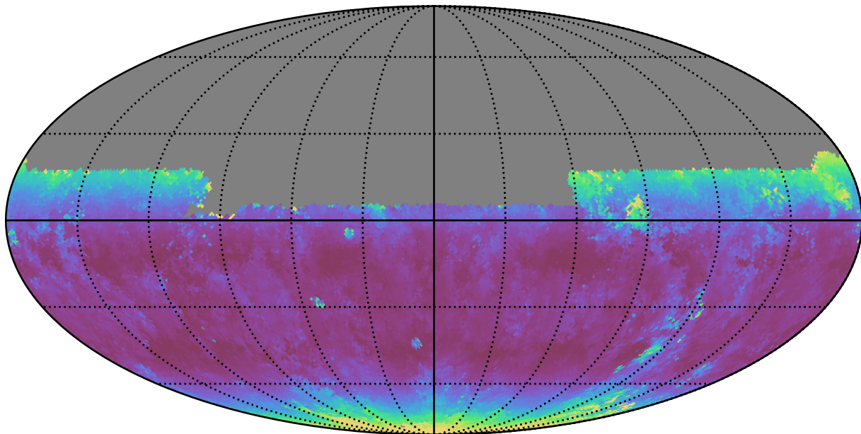
early_u_fpextra3.0_v3.4_10yrs Yr 1 y band: Median airmass
